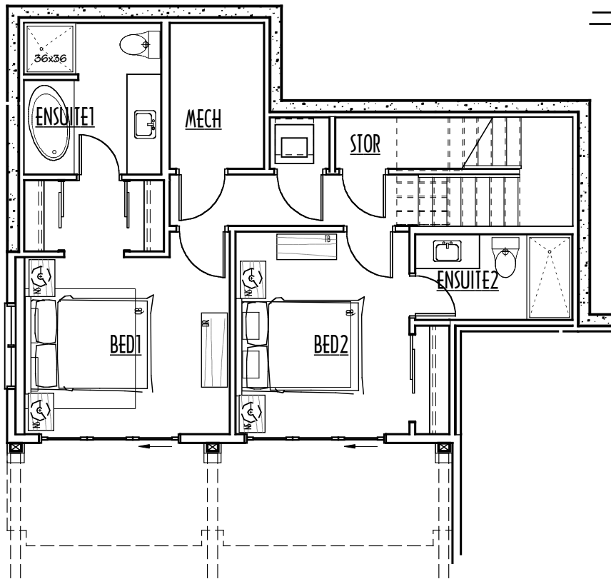
FURNITURE PLAN QUARRY BAY F1 GROUND LEVEL
