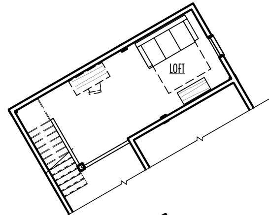
FURNITURE PLAN QUARRY BAY D2 ROOF TOP
