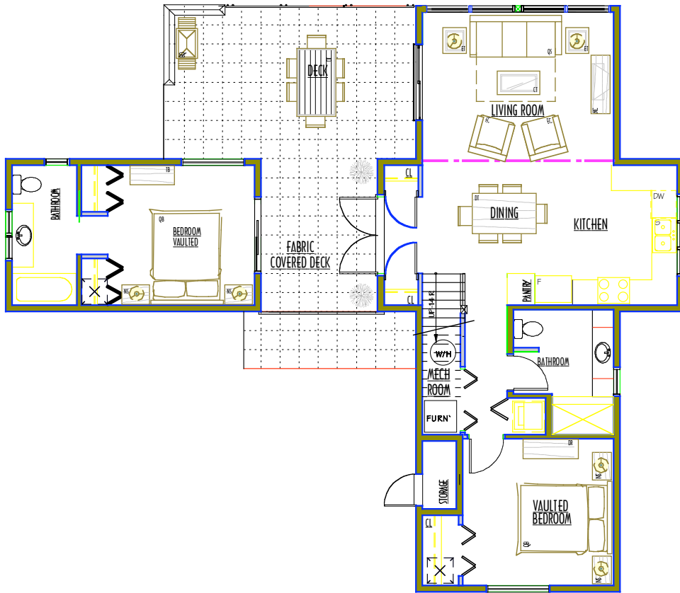
FURNITURE PLAN FORREST CABIN #3 MAIN FLOOR
